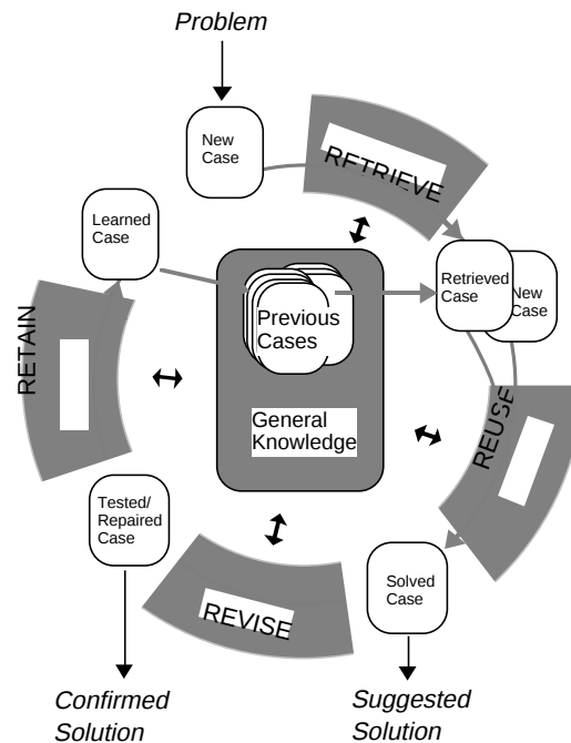
Fig. 1. The case-based reasoning cycle [AaPl94]
